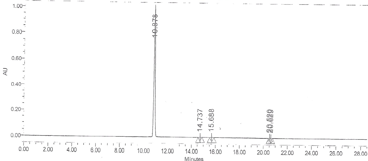
Auto-Scaled Chromatogram
